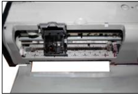
Open the printer cover, move the cartridge Carriage to "cartridge replace position", And take out the original cartridges.
