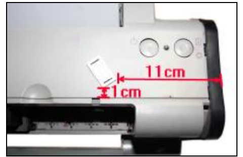
Fix the supporting arm as the picture shows. Measure 11 cm from the right edge of printer, 1 cm from the below edge, which forms an angle of 60 degree.
